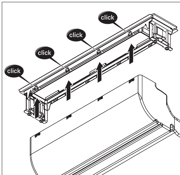
Fig. 6.22 Feste modulen for undermontering
