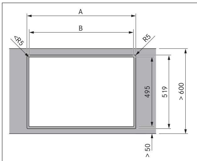
Fig. 6.2 Planlimt montering
